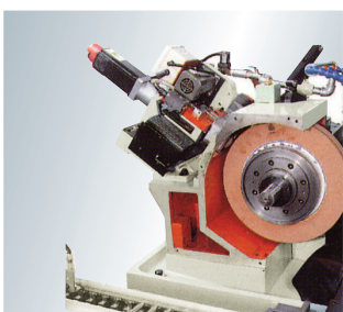
⑯ Rotary type grinding wheel dressing attachment
