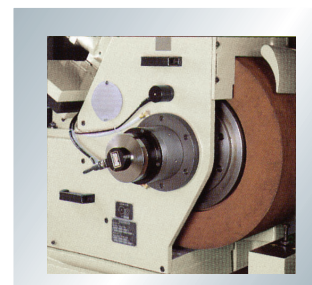
⑮ Grinding wheel automatic balancing system
