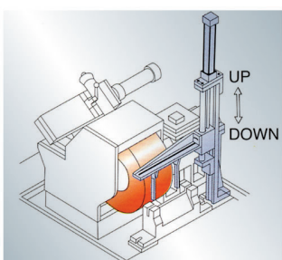
⑦ Manual parts feeder for infeed grinding
