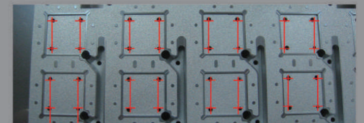
Repeatability 2μm WAFER BUMPING MOLD
