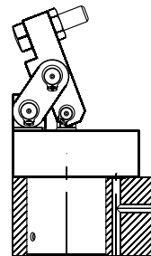
Type B Plug-in design, oil supply manifold with O-ring
