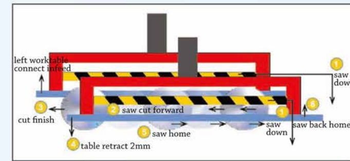
SAWBLADE FEED WAY DIAGRAM
