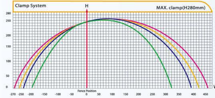
BMT 2036 Cutting Capacity Chart
