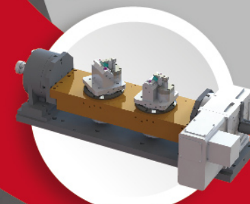
4+1 軸油壓轉台 / 夾治具 4+1-axis Hydraulic Rotary Unit / Jig And Fixture
