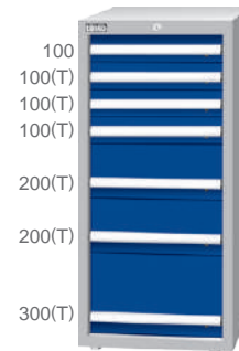
EA-12074(T) W566xD607xH1200 EB-12074(T) W718xD607xH1200 ED-12074(T) W718xD759xH1200
