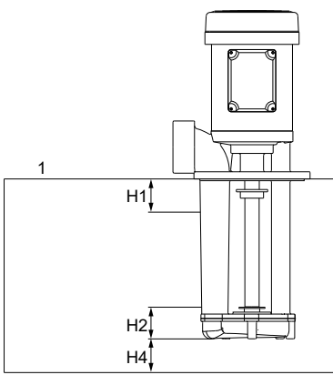
MTA with bottom inlet
