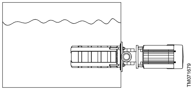
Horizontally installed MTR version H pump
