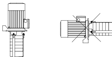
Installation of an MTH pump. Left: vertical. Right: horizontal
