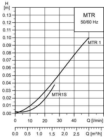
Pressure losses of pumped liquid passing through an empty chamber for MTR 1s and MTR 1 pumps
