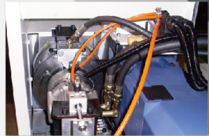
▲ 副主軸吹氣及推料裝置 Air-blowing and finished parts ejector device for Sub-spindle
