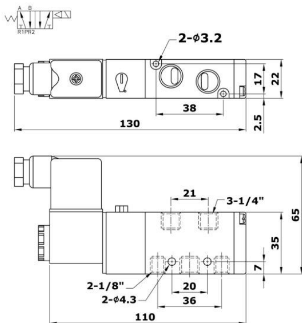
NA212-Operation Single Type Drawing
