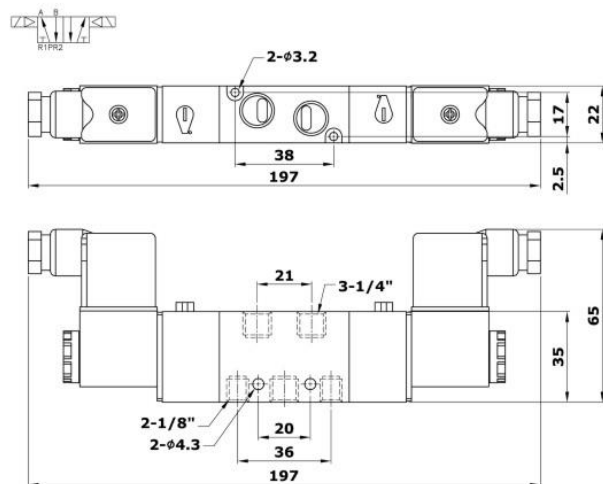
NA212-Operation Double Type Drawing
