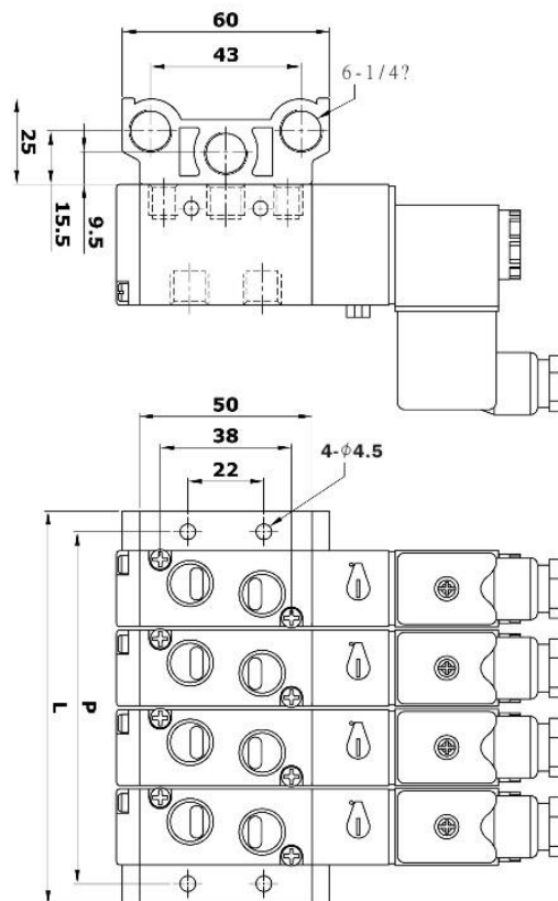
NA212-Manifold Type Drawing
