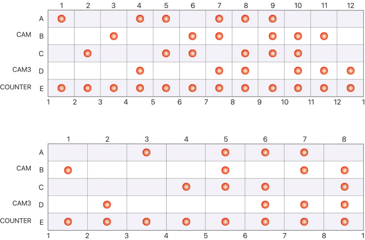
Electrical Sequence Diagram CLT-63, 80, 100, 125, 200, 300
