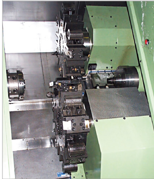
CLT-100-12T + CLT-100L-12T (Hydraulic Turret)
