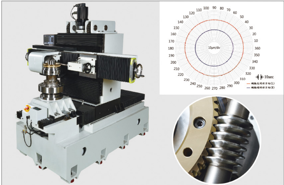
Suface Contact and Pitch Error Testing for Worm Gear System.
