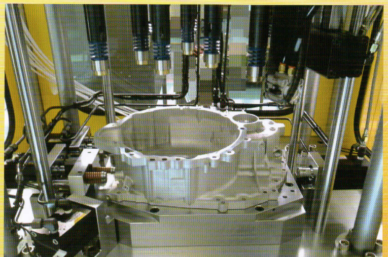
單工乾式壓檢機(測漏機) Dry type in one leaking testing machine
