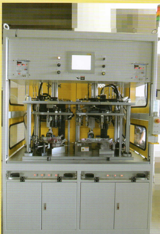
雙工乾式壓檢機(測漏機) Dry type in one leaking testing machine
