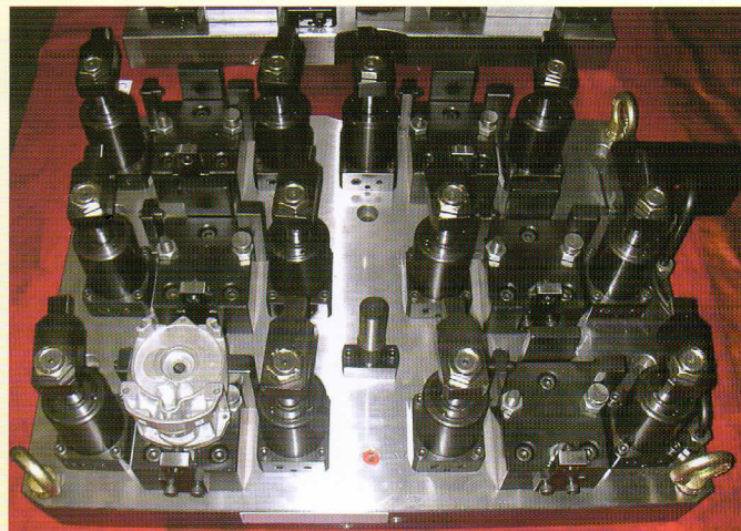
立式M/C用油壓治具 Hydraulic Fixtures
