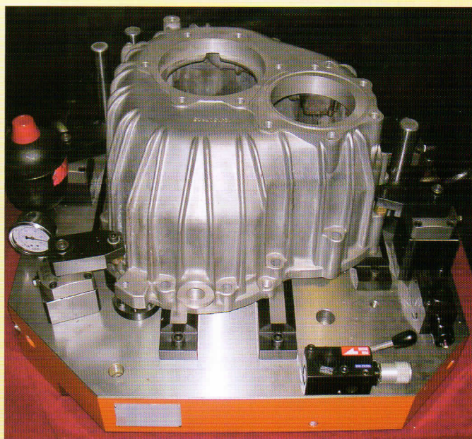
油壓保壓治具 Hydraulic Fixtures with the Accumulator
