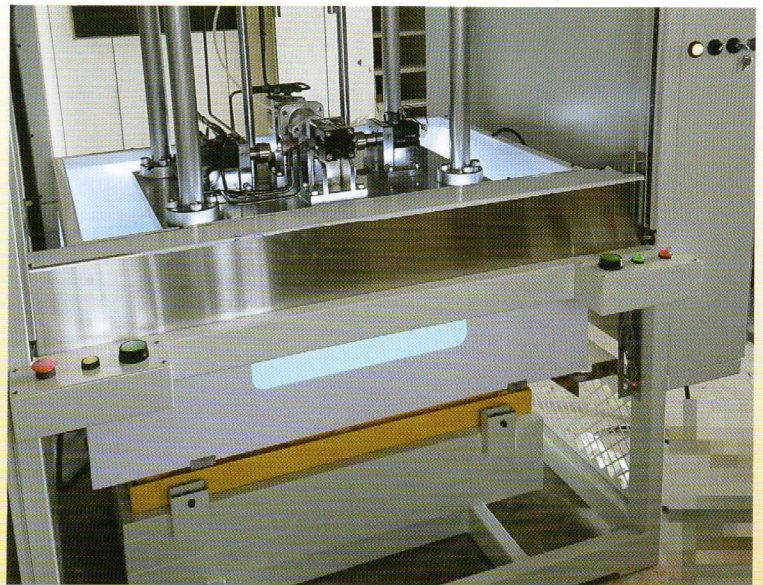
升降式照明水箱(便於肉眼辨識試漏位置) Lifting water tank with lights
