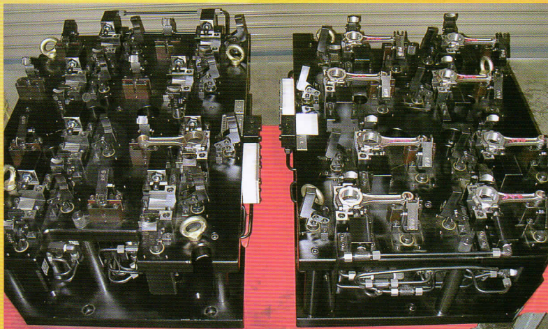
立式M/C用油壓治具 Hydraulic Fixtures
