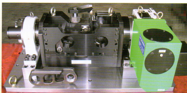
轉台用油壓治具 Indexing Fixtures
