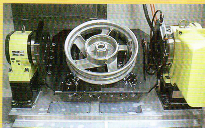
轉台用油壓治具 Indexing Fixtures
