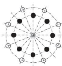
16刀 - 雙PCD 16Pos. - 2 graduated circles
