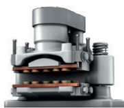
EMB-STOP S-A-xx-F
