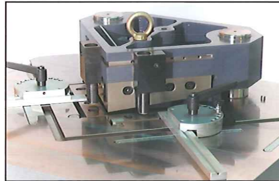
STURDY WORKHEAD, CONICAL GROOVES WITH SET OF GONIOMETRY SQUARES ON RIGID CAST IRON WORKTABLE.
