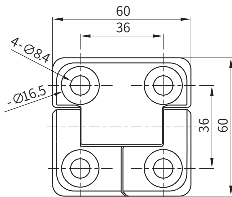
M8鑲嵌螺柱 With Threaded Studs M8
