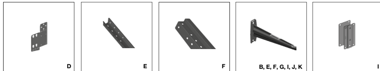
Top Corner Bracket Item No. 7700-066 Used together with Post Bracket (7700-014) for mounting in the corner at the top of the post (D). Incl. screw and plug. Bracket Holder Item No. 7700-032 Used together with X15 Bracket for mounting on top of the post 50x50 (E). Bracket Holder 70x70 Item No. 7700-188 Used together with X15 Bracket for mounting on top of the post 70x70 (F). X15 Bracket Item No. 2715-Length Comes in 4 different lengths 120, 220, 320 & 420 mm. Can be mounted on Corner Bracket (B), Bracket Holder 50x50 (E), Bracket Holder Aluminium (G) and 70x70 (F), Adjustable Post Fitting (I), Adjustable Corner Post Fitting (J) and Post Bracket Holder (K). Adjustable Post Fitting Item No. 7700-060 Optional placement on the post for mounting the X15 Bracket (I). Incl. bolts and nuts.
