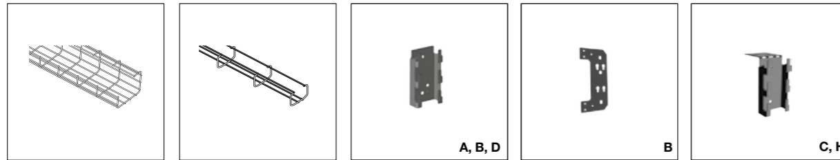
X-Tray G 120x150x2300 Item No. 1722-2300 X-Tray Mini 30x22x2300 Item No. 1752-2300 X-Tray Mini 30x22x1200 Item No. 1752-1200 Post Bracket Item No. 7700-014 Corner Bracket Item No. 7700-065 Post Bracket Top Item No. 7700-015 Mounted in the key holes on the post (A). Used together with the Corner Bracket (7700-065) for inside corners (B) and together with Top Corner Bracket (7700-066) for inside corners at the top of the post (D). Used in corners together with the Post Bracket (7700-014) (B). Can also be used elsewhere on the post, also the X15 Bracket can be mounted onto it. To be mounted at the top of the post (C). For wire trays in sizes of 60-120 mm. If the upper part is straightened out 90° it can be mounted anywhere on the post (H). Incl. screw and plug.
