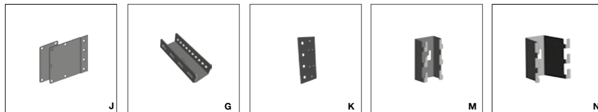
Adjustable Corner Post Fitting Item No. 7700-072 Optional placement on the corner post for mounting the X15 Bracket (J). Incl. bolts and nuts. Bracket Holder Aluminium Rail Item No. 7700-037 Mount the X15 Bracket onto the aluminium rail above sliding doors (G). Fits together with wire trays mounted with X15 Bracket on top of the posts with Bracket Holder. Incl. bolt and nuts. Post Bracket Holder Item No. 7700-083 Mount the X15 Bracket at the post, using the key holes (K). Mesh Panel Mini Bracket Item No. 7700-084 For mounting onto the mesh panel (M). Mesh Panel Bracket Item No. 7700-090 For mounting onto the mesh panel in line with wire trays mounted with Post Bracket (7700-014) (N).
