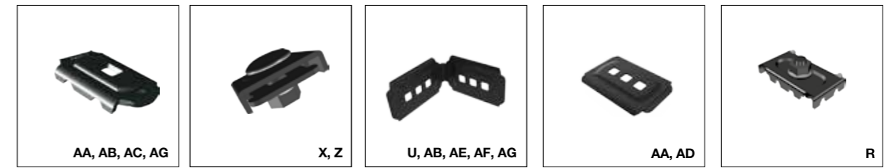
X1 Fitting Item No. 2701 Used with X3 Angled Fitting or to mount the wire trays with another item, as for example an X14 Pendant or X15 Bracket. When assembling a corner (T) or an reduction (V) X1 Fittings also are used. X2 Fitting Item No. 2702 When forming the wire tray, the X2 Fitting are used for radius (Z) or when doing a vertical decline from a horizontal wire tray (X). X3 Angled Fitting Item No. 2703 For T-crossings (AB) or connections to the wall or floor (AG). To adjust the angle some degrees (U). Can also be used mount vertical wire trays onto horizontal wire trays (AE) (AF). X4 Fitting Item No. 2704 When mounting wire trays at the top of the post the X4 Fitting can be used together with the X1 Fitting to raise the wire tray above the hinge door (AA). Used to mount a vertical wire tray underneath a horizontal wire tray (AD). X5 Joining Fitting Item No. 2705 20 pcs, incl. bolt and nut. For joining the wire trays. Bracket mounted on the outside and bolt from the inside.
